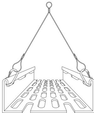
2. Link hook Y-Fit on cable tray.
