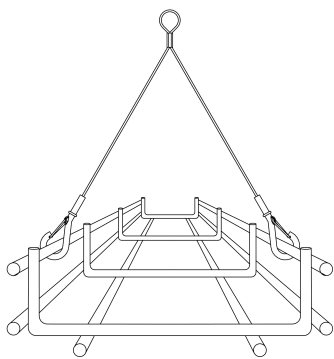
1. Snap Hook in Y-Fit on cable basket.
