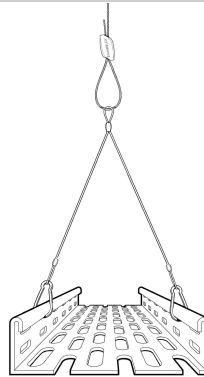
3. Karabiner Y-Fit accessory and Gripple Loop hanger kit on cable tray.
