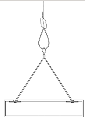
4. Toggle Y-Fit Accessory with Gripple hanger.
